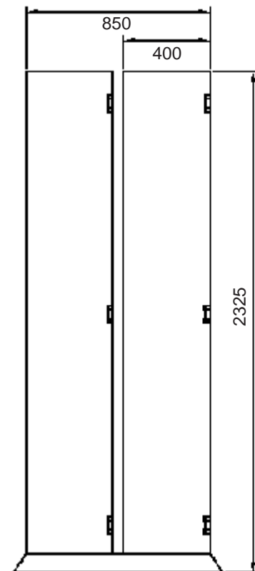
Side view of double unit
